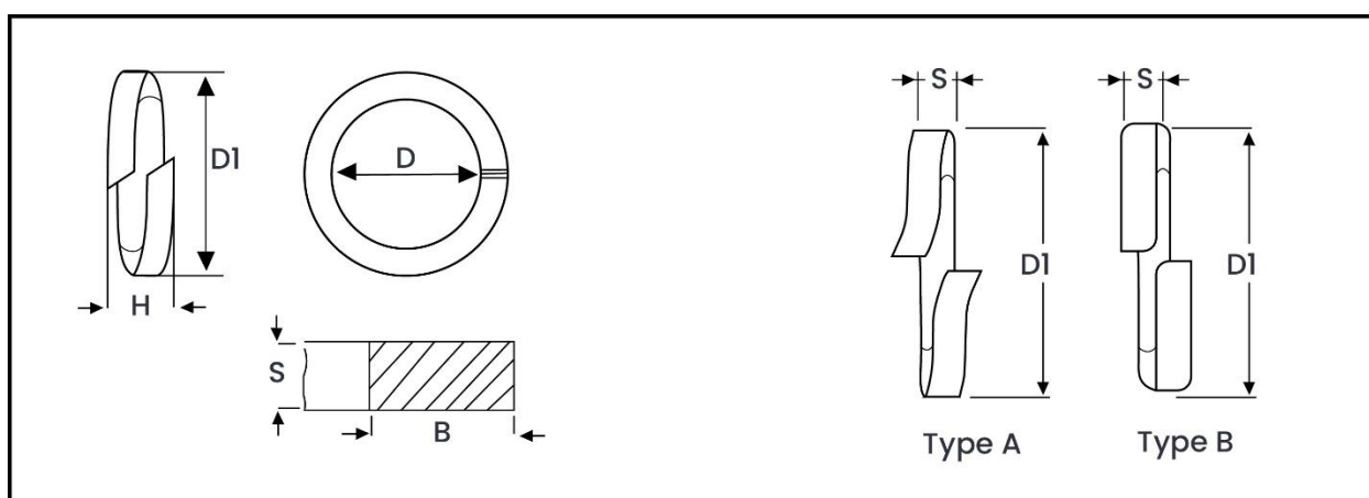
Metric Dimensions – DIN 127 Helical Spring Lock Washer
