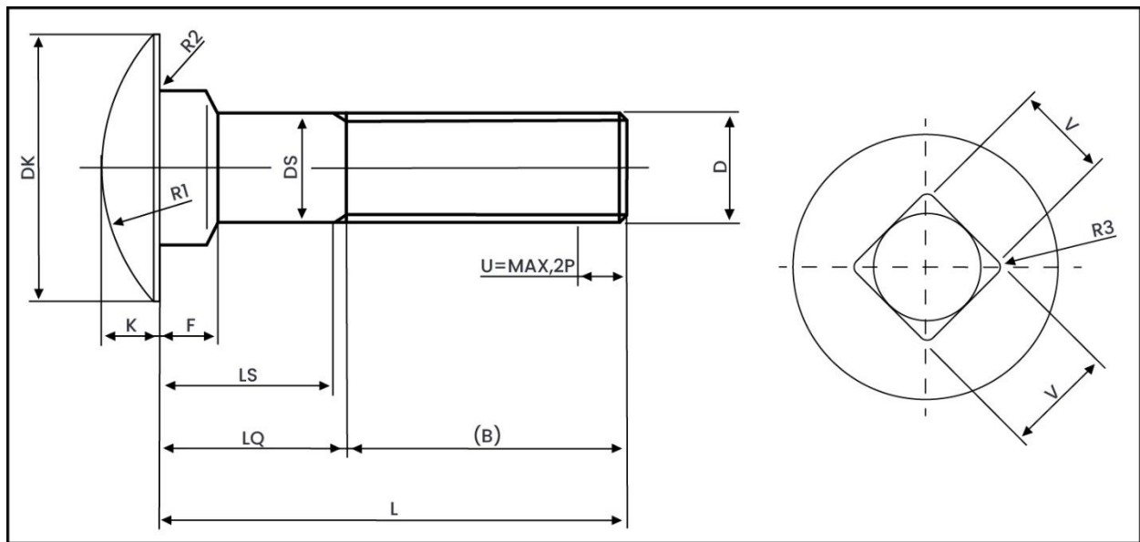
Metric Dimensions – DIN 603 Carriage Bolt – Round Head Square Neck
