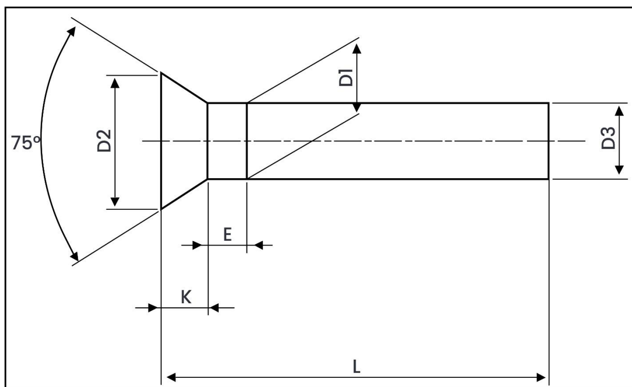
Metric Dimensions – DIN 661 Countersunk Head Rivet
