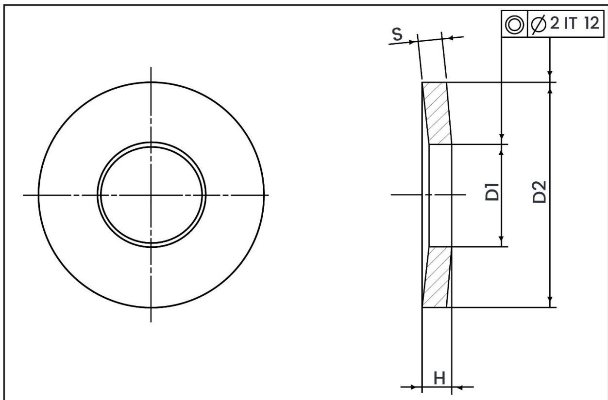
Metric Dimensions – DIN 6796 Conical Spring Washer
