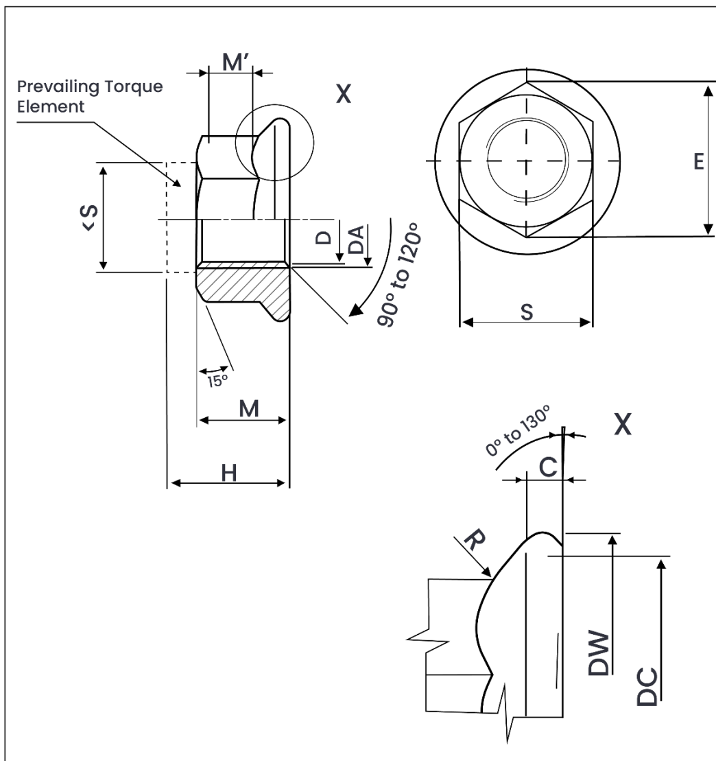
Metric Dimensions – DIN 6926 Flange Nylock Nut
