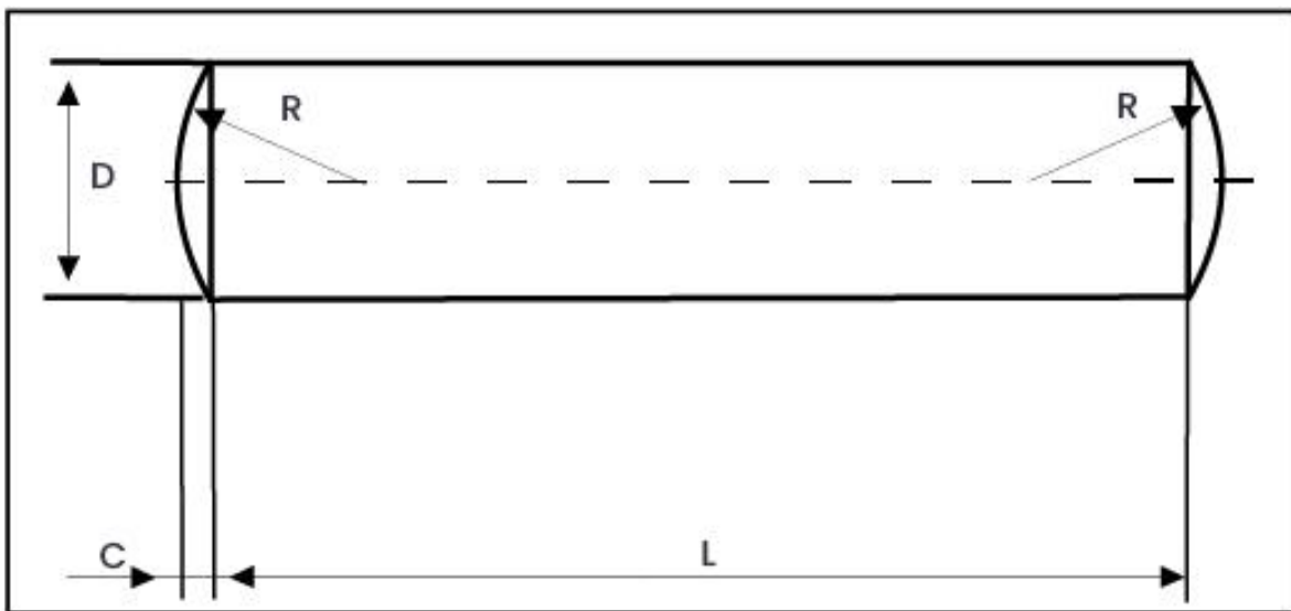
Metric Dimensions – DIN 7 Parallel Dowel Pin
