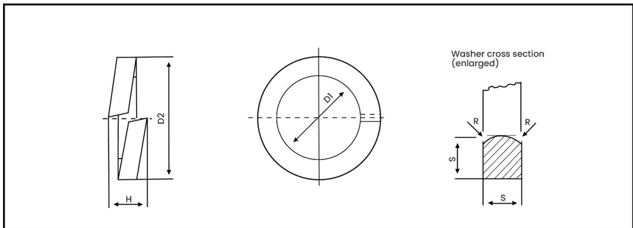
Metric Dimensions – DIN 7980 Spring Lock Washer with Square End
