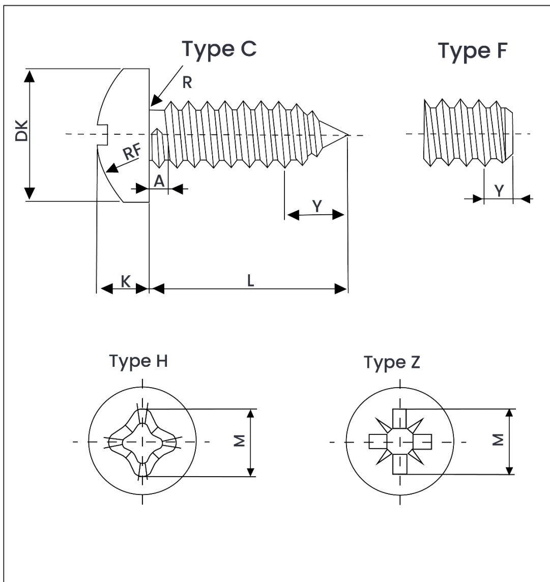
Metric Dimensions – DIN 7981 Cross Recessed Pan Head Tapping Screw
