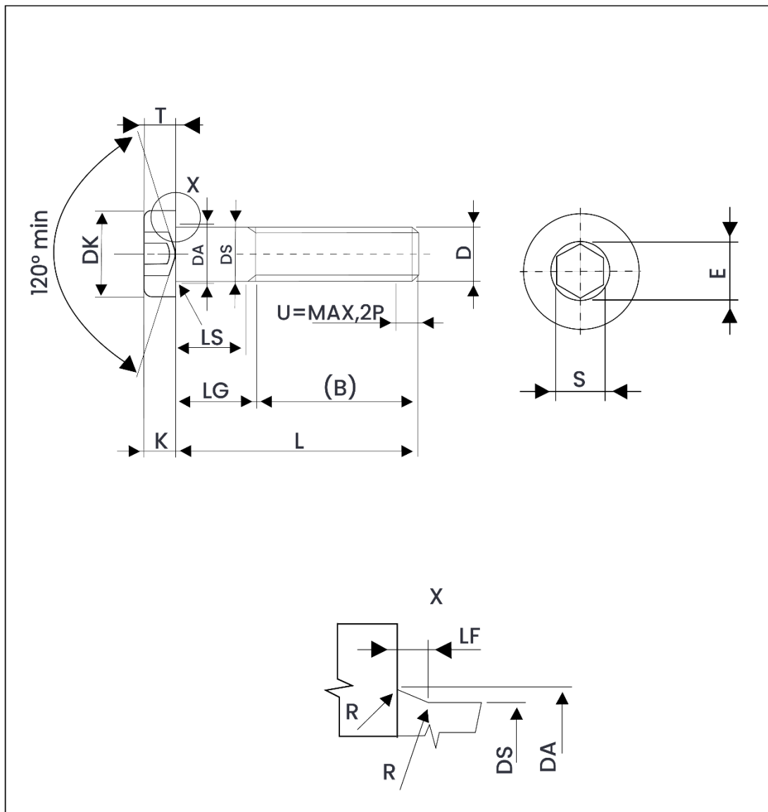
Metric Dimensions – DIN 7984 Low Head Socket Cap Screw
