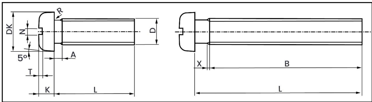
Metric Dimensions – DIN 85 Slotted Pan Head Screw
