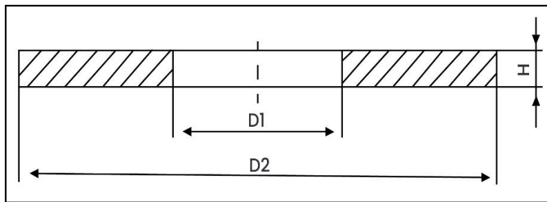
Metric Dimensions – DIN 9021 Large Size Flat Washer
