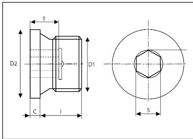
Metric Dimensions – DIN 908 Hexagon Socket Screw Plugs with Sealing Face
