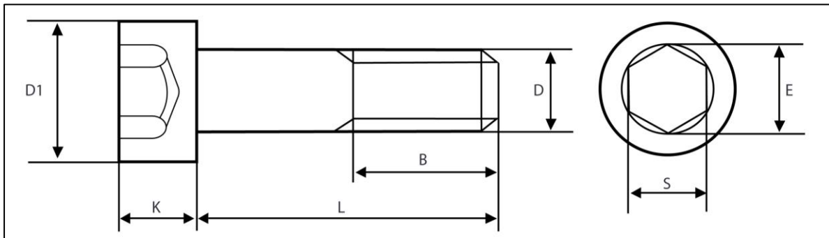
Metric Dimensions – DIN 912 Hexagon Socket Head Cap Screw
