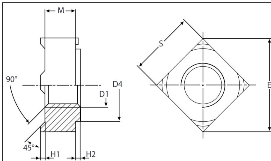
Metric Dimensions – DIN 928 Square Weld Nut
