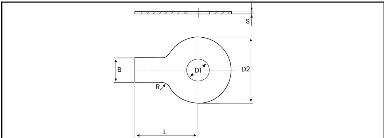
Metric Dimensions – DIN 93 Tab Washer with Long Tab
