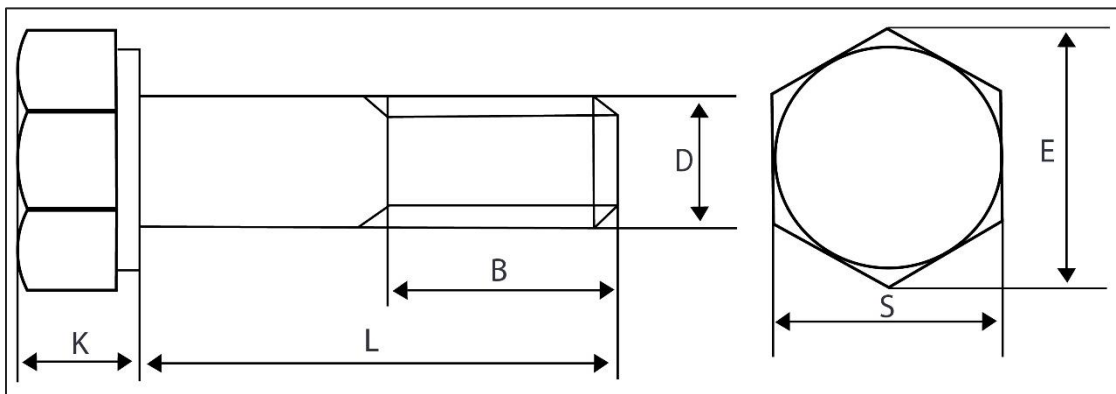
Metric Dimensions – DIN 931 Hexagon Head Bolt (Partially Threaded)
