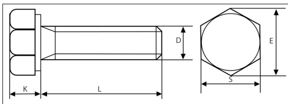
Metric Dimensions – DIN 933 Hexagon Head Bolt (Fully Threaded)
