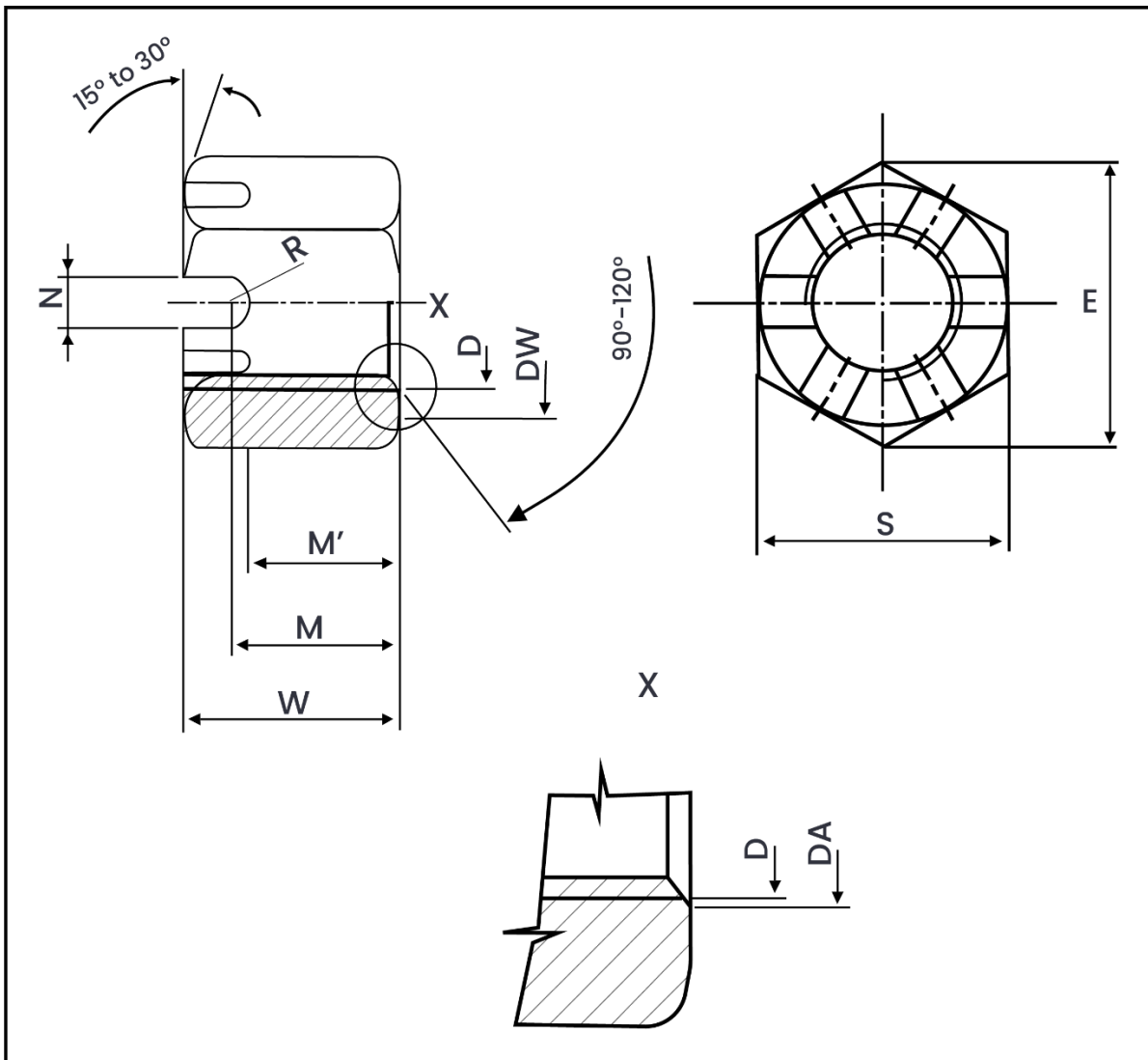
Metric Dimensions – DIN 935 Slotted Hex Castle Nut
