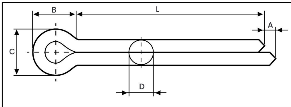
Metric Dimensions – DIN 94 Split Pin (Cotter Pin)
