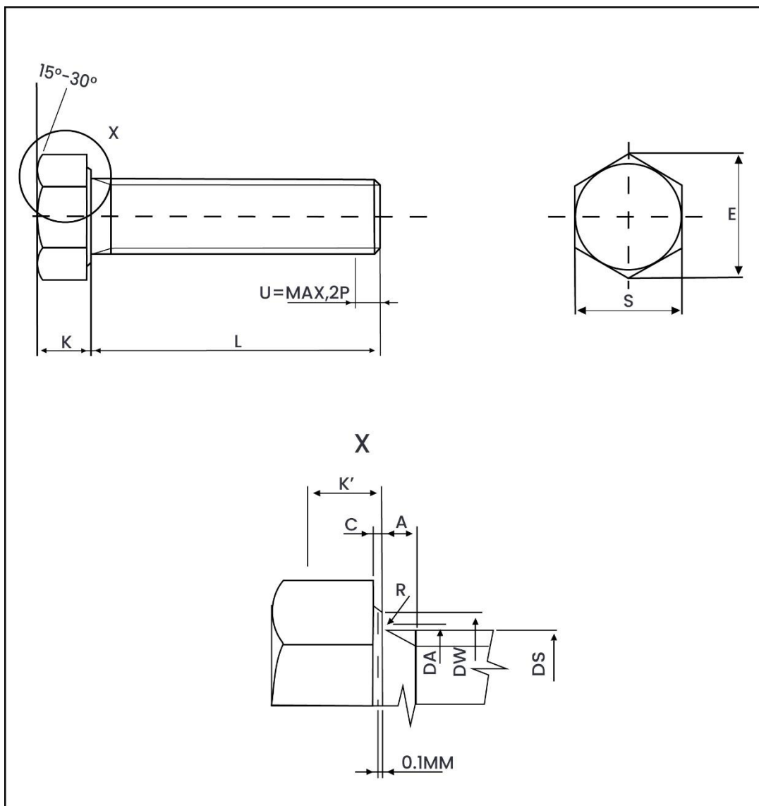
Metric Dimensions – DIN 961 Hex Bolt (Fully Threaded)
