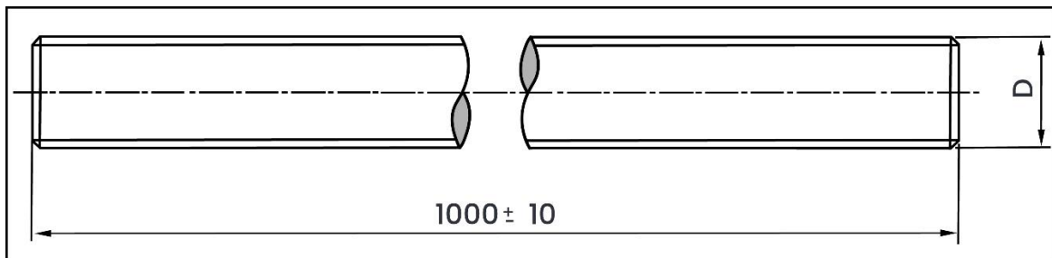
Metric Dimensions – DIN 975 Threaded Rod
