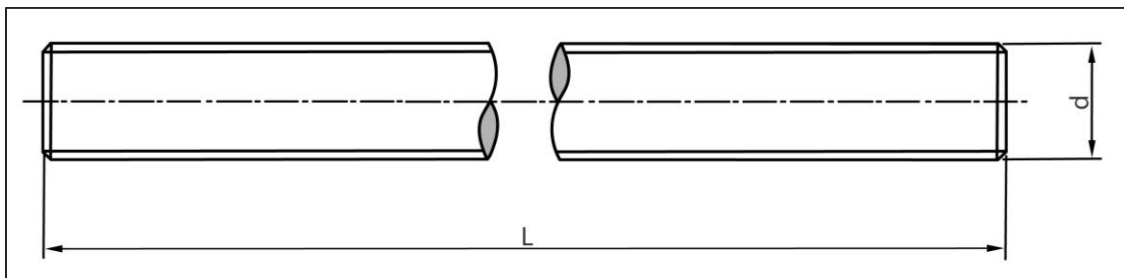
Metric Dimensions – DIN 976 Threaded Rod (Stud)
