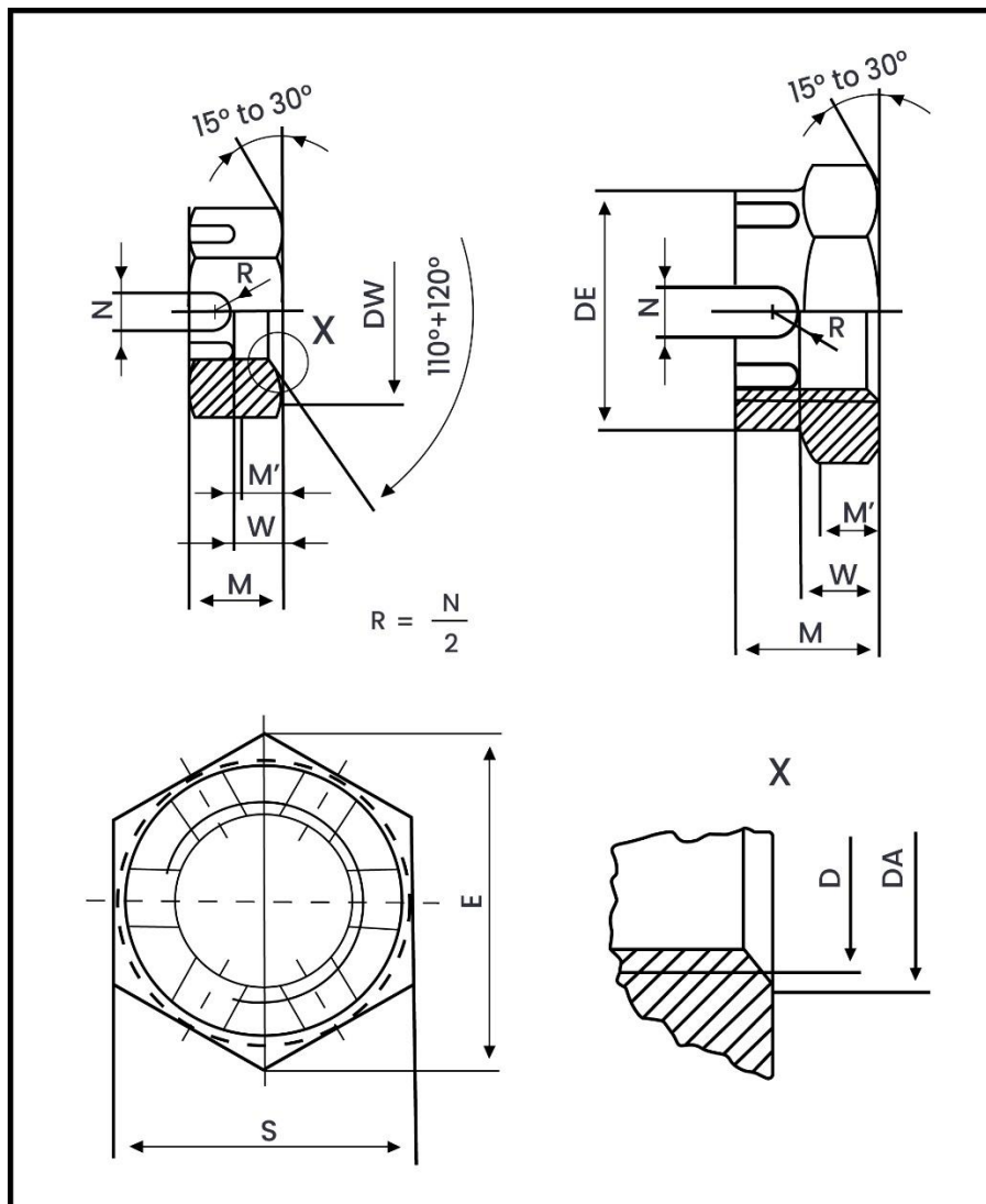
Metric Dimensions – DIN 979 Thin Hexagon Slotted Castle Nut
