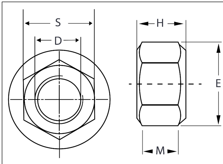
Metric Dimensions – DIN 982 Hex Lock Nut with Nylock Insert
