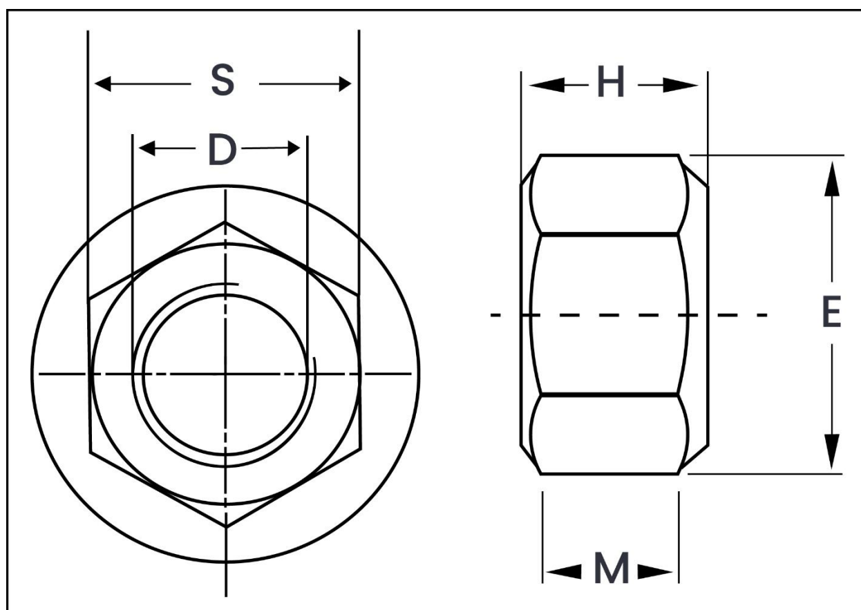
Metric Dimensions – DIN 985 Low Hex Lock Nut with Nylock Insert
