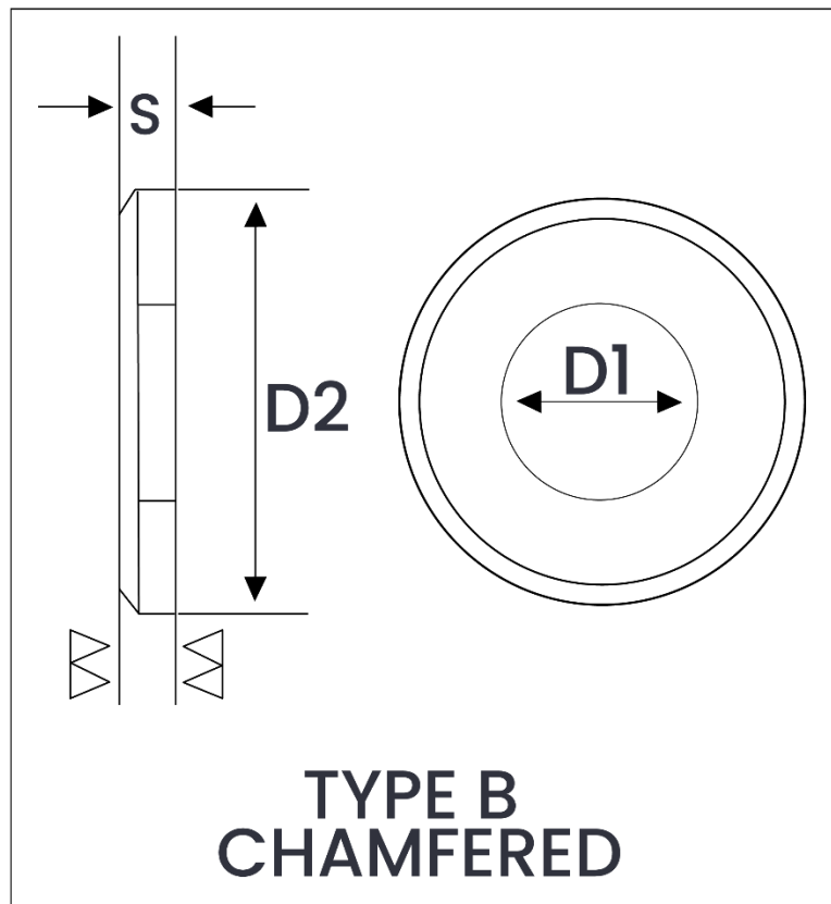
Weight Chart – DIN 125B Flat Washer – Form B (With Chamfer)
