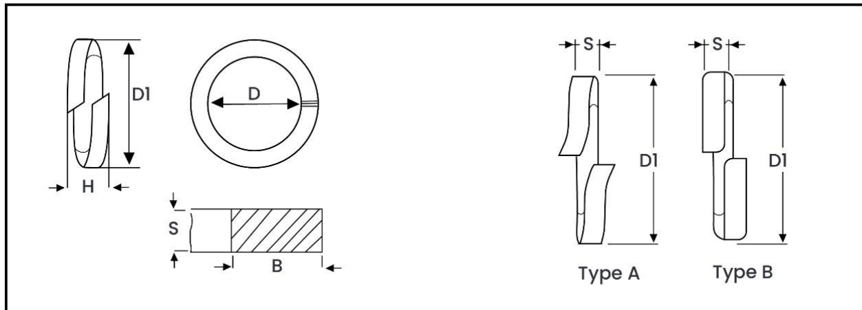
Weight Chart – DIN 127 Helical Spring Lock Washer
