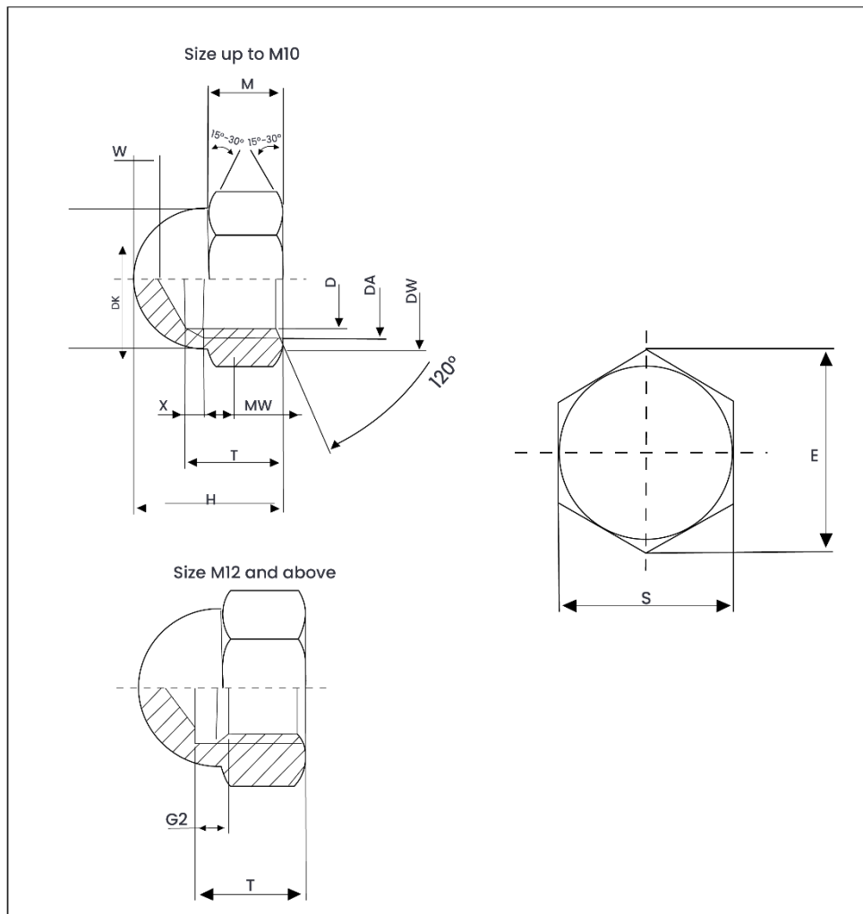
Weight Chart – DIN 1587 Hexagon Domed Cap Nut
