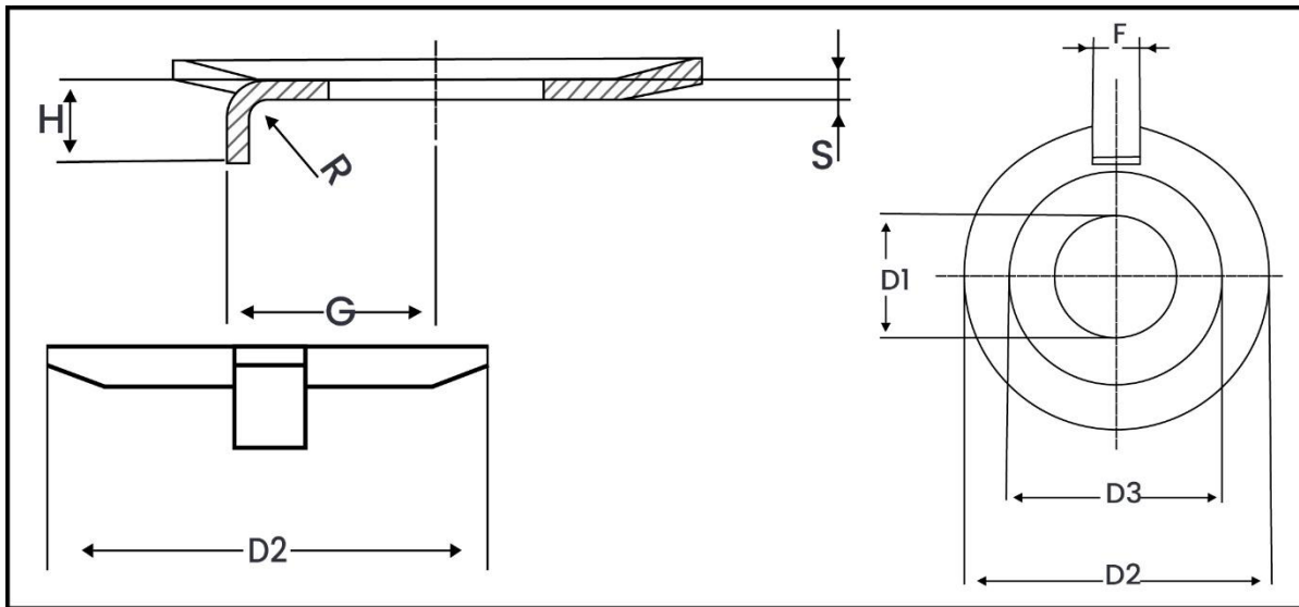
Weight Chart – DIN 432 External Tab Washer
