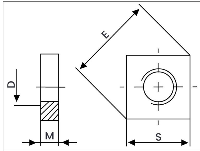
Weight Chart – DIN 562 Thin Square Nut
