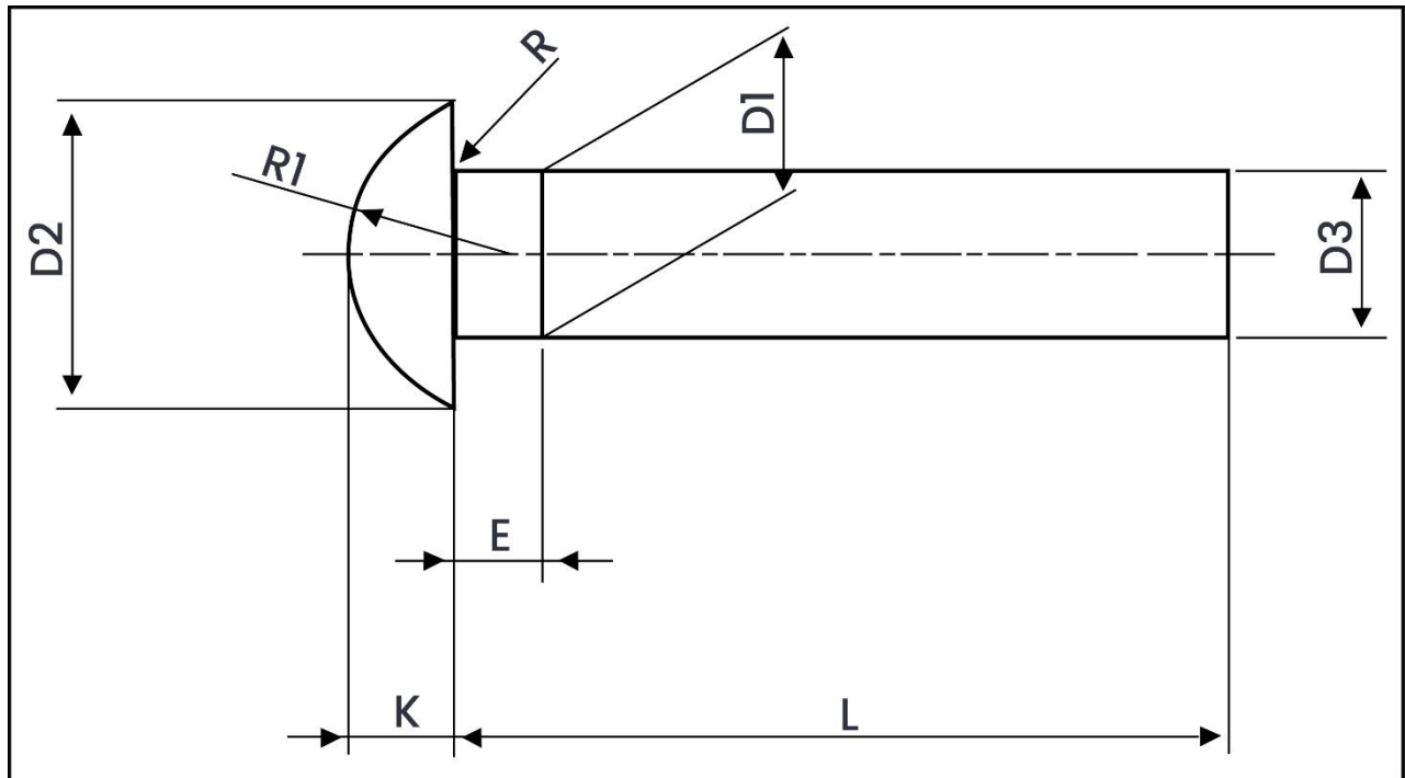
Weight Chart – DIN 660 Round Head Rivet
