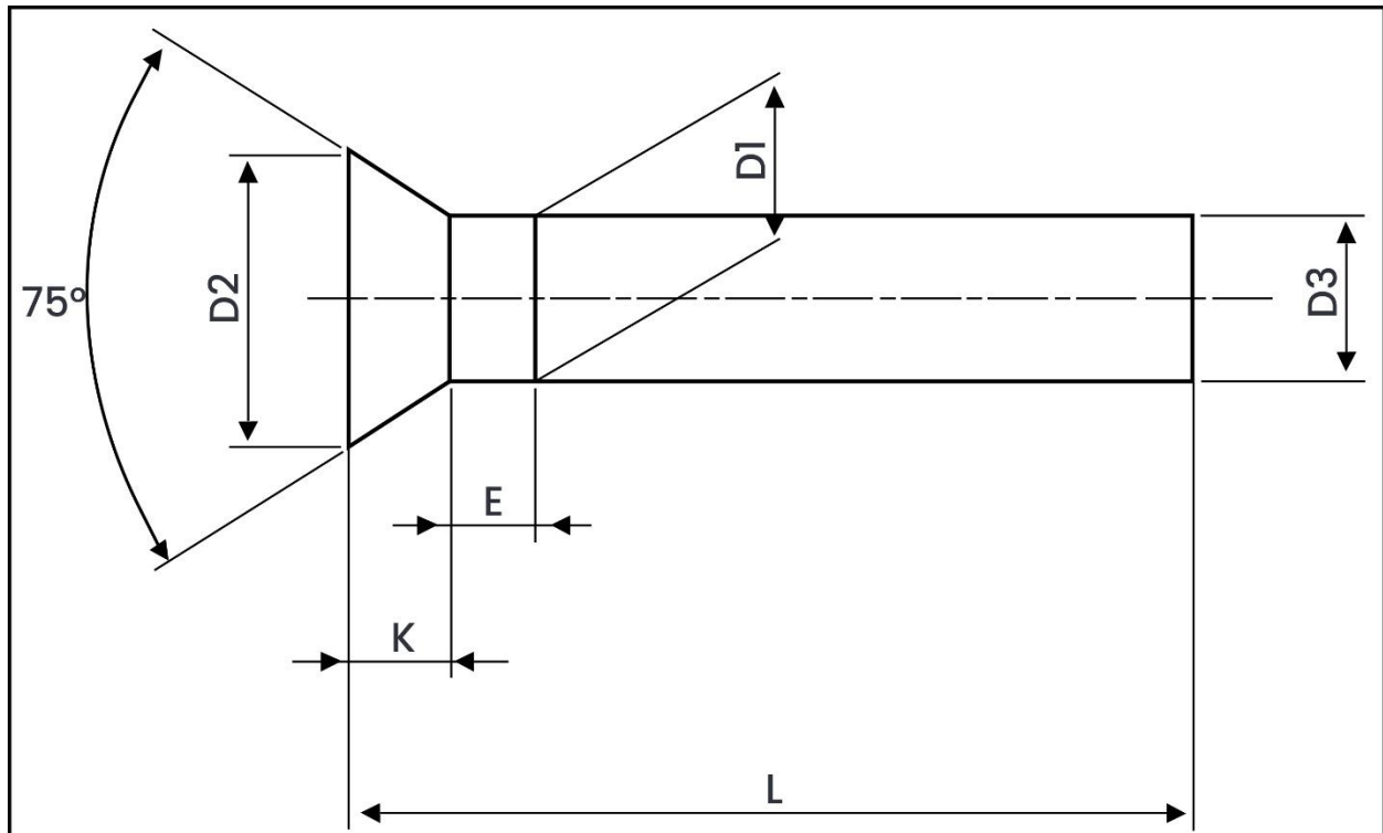
Weight Chart – DIN 661 Countersunk Head Rivet
