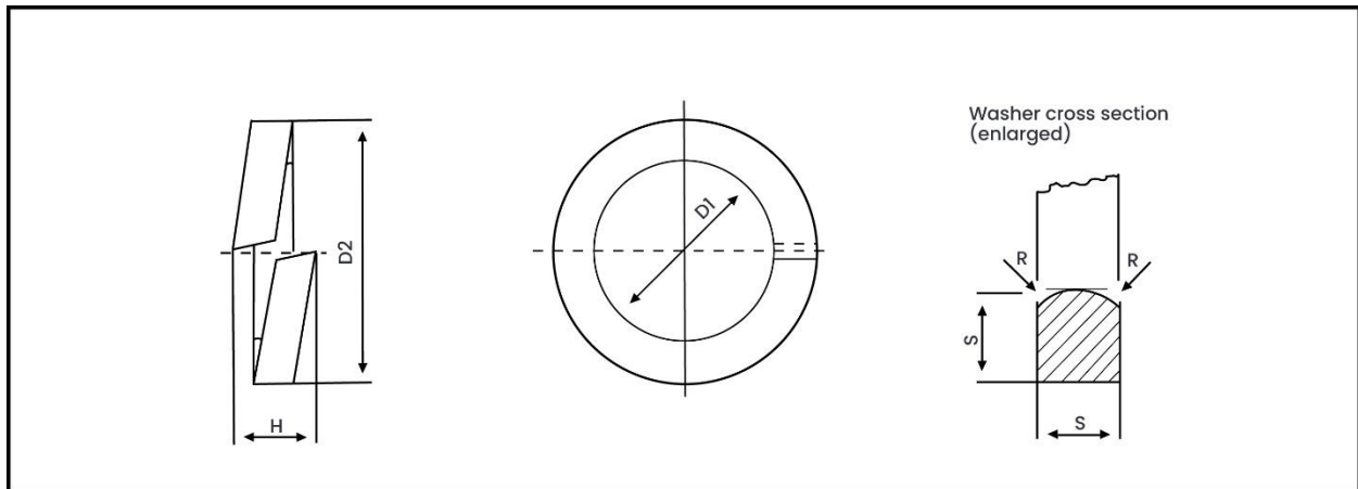
Weight Chart – DIN 7980 Spring Lock Washer with Square End
