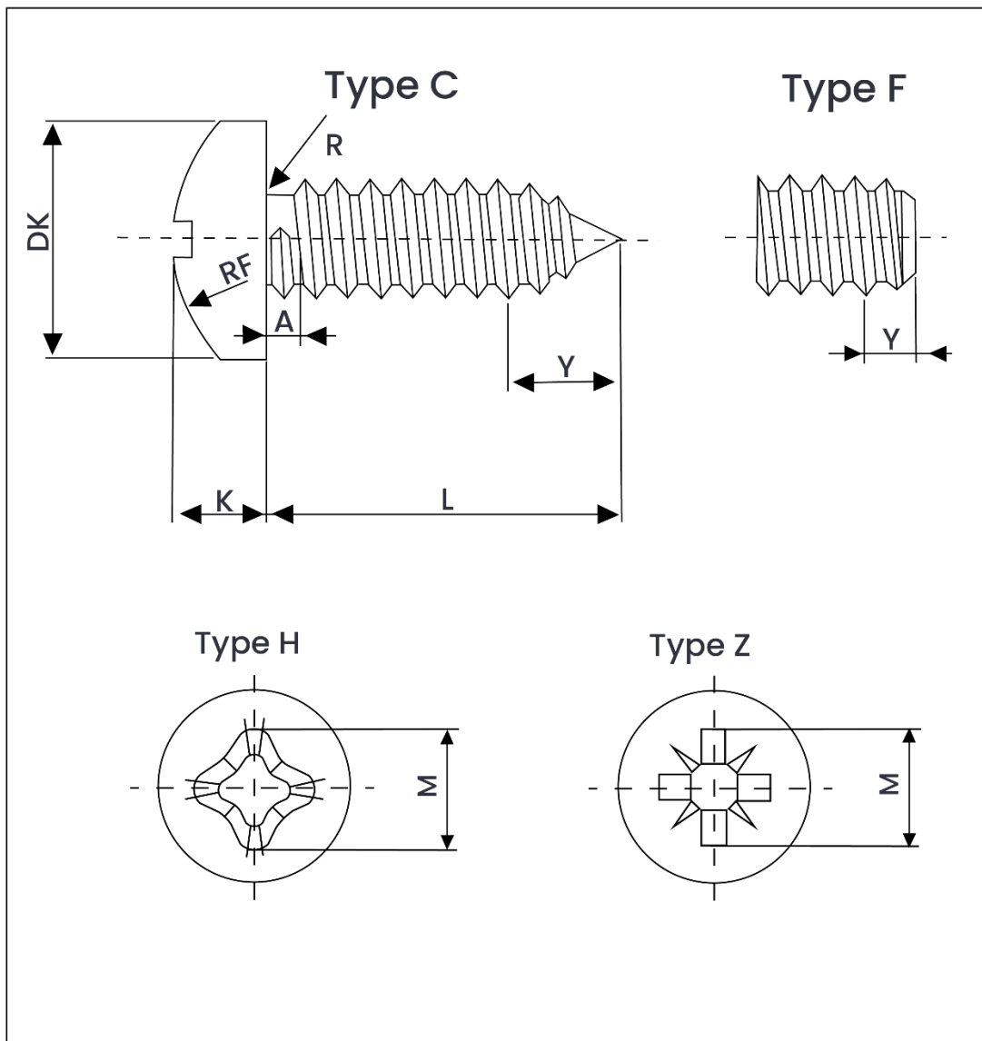
Weight Chart – DIN 7981 Cross Recessed Pan Head Tapping Screw
