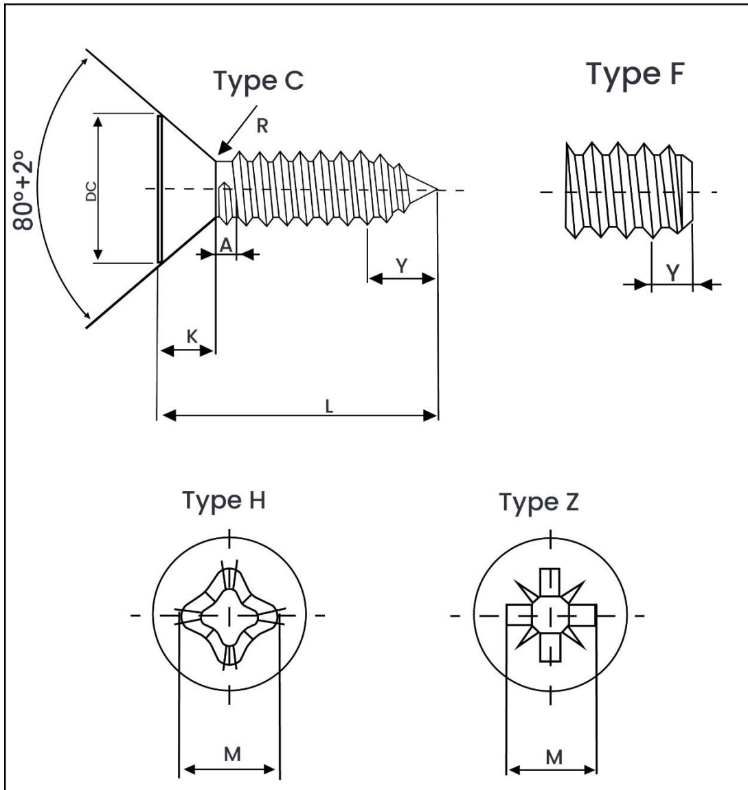
Weight Chart – DIN 7982 Cross Recessed Countersunk Head Tapping Screw
