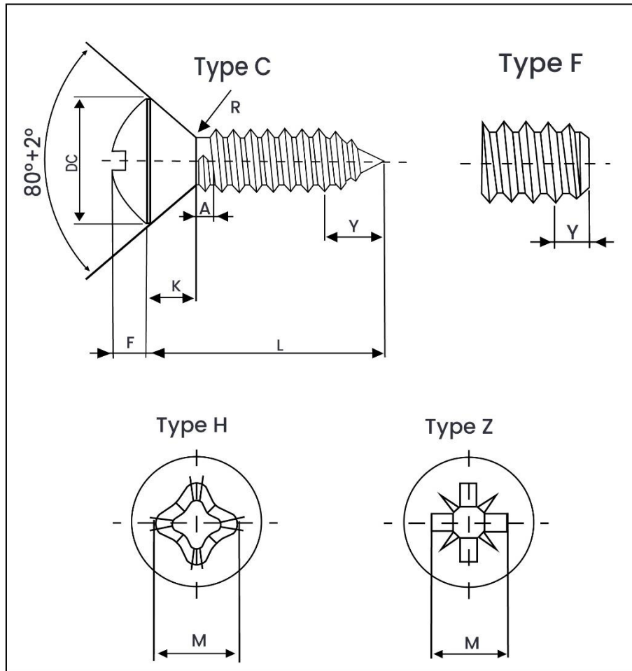
Weight Chart – DIN 7983 Cross Recessed Raised Countersunk Head Tapping Screw
