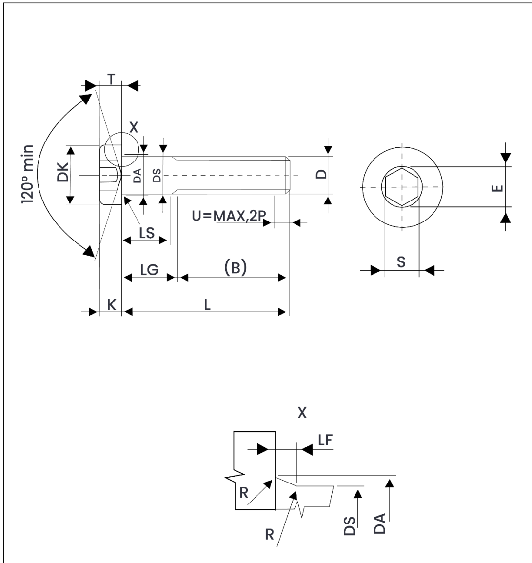
Weight Chart – DIN 7984 Low Head Socket Cap Screw
