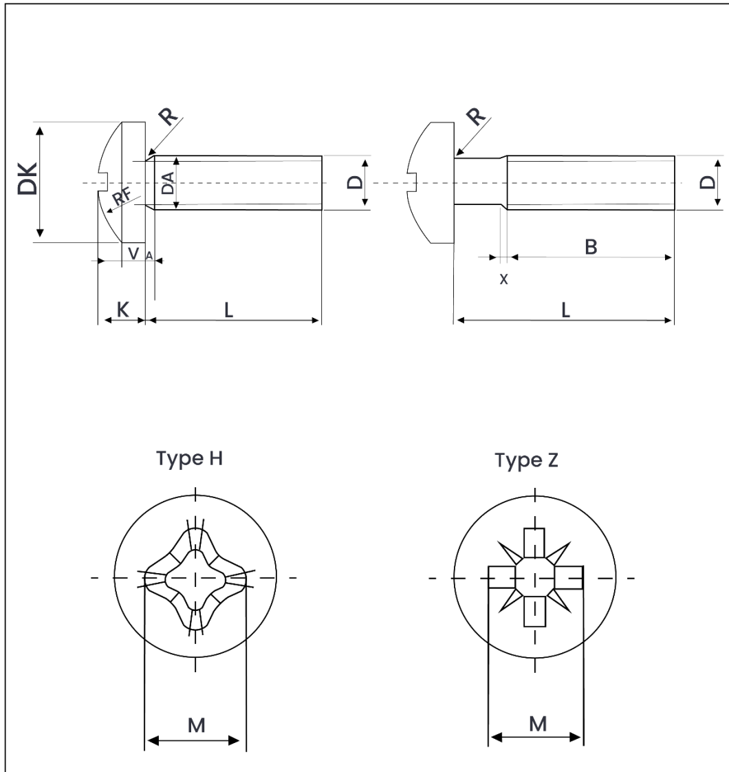
Weight Chart – DIN 7985 Cross Recessed Pan Head Screw
