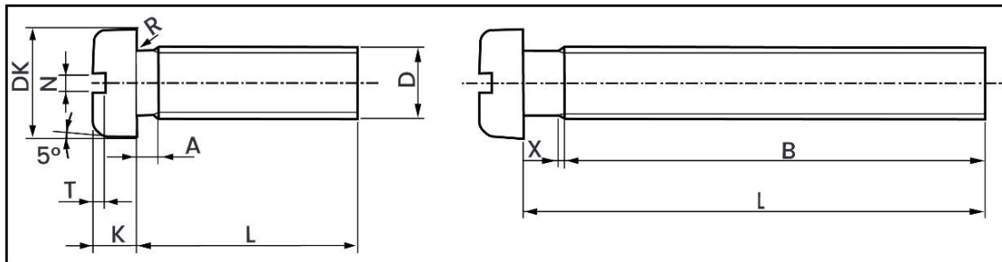
Weight Chart – DIN 84 Slotted Cheese Head Screw
