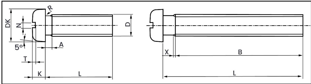
Weight Chart – DIN 85 Slotted Pan Head Screw
