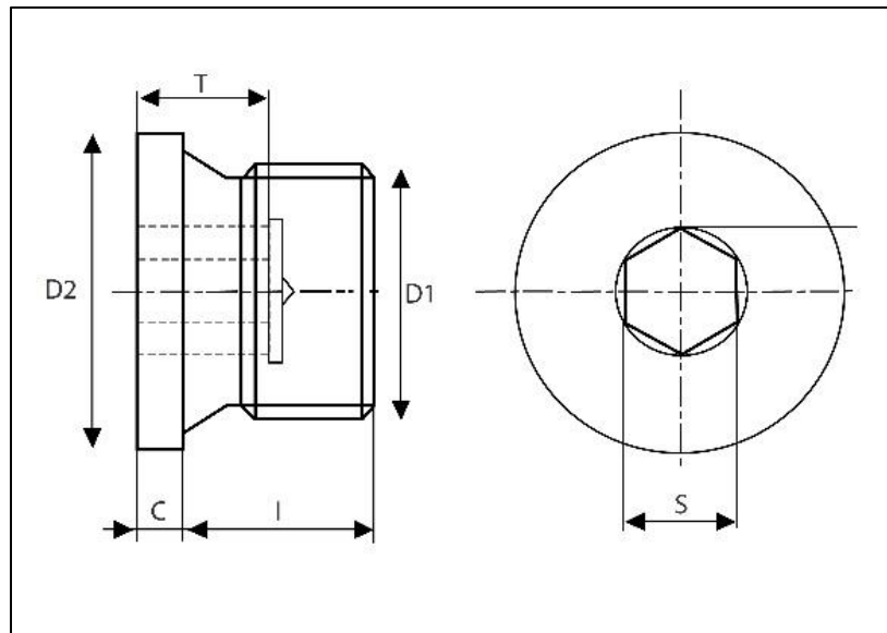
Weight Chart – DIN 908 Hexagon Socket Screw Plugs with Sealing Face
