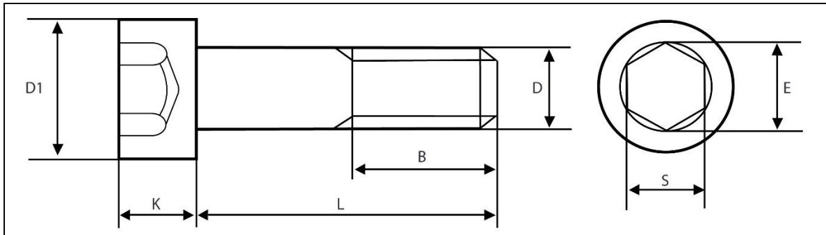
Weight Chart – DIN 912 Hexagon Socket Head Cap Screw
