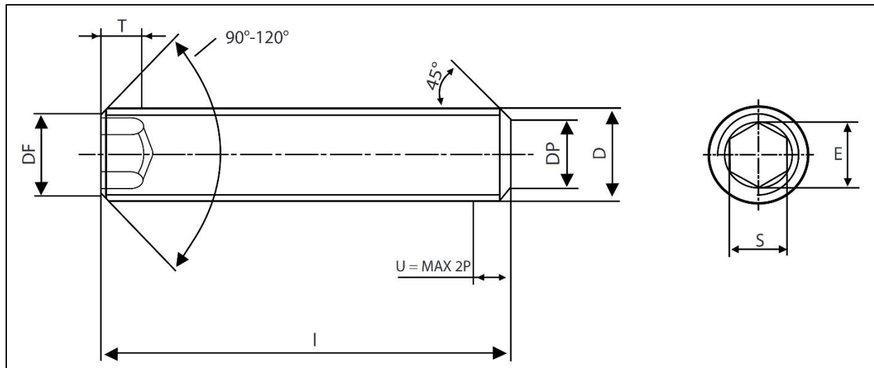
Weight Chart – DIN 913 Hexagon Socket Set Screw with Flat Point
