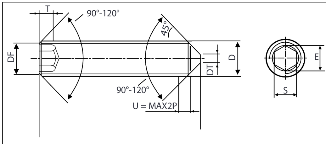
Weight Chart – DIN 914 Hexagon Socket Set Screw with Cone Point
