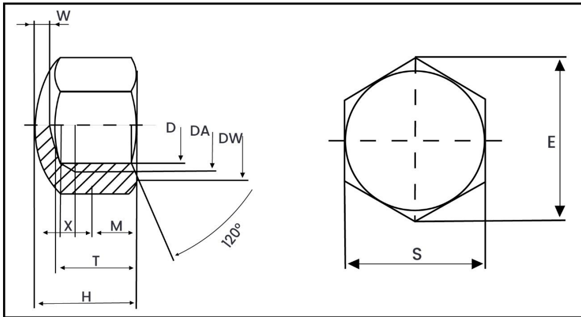
Weight Chart – DIN 917 Hexagon Domed Cap Nut (Low Type)
