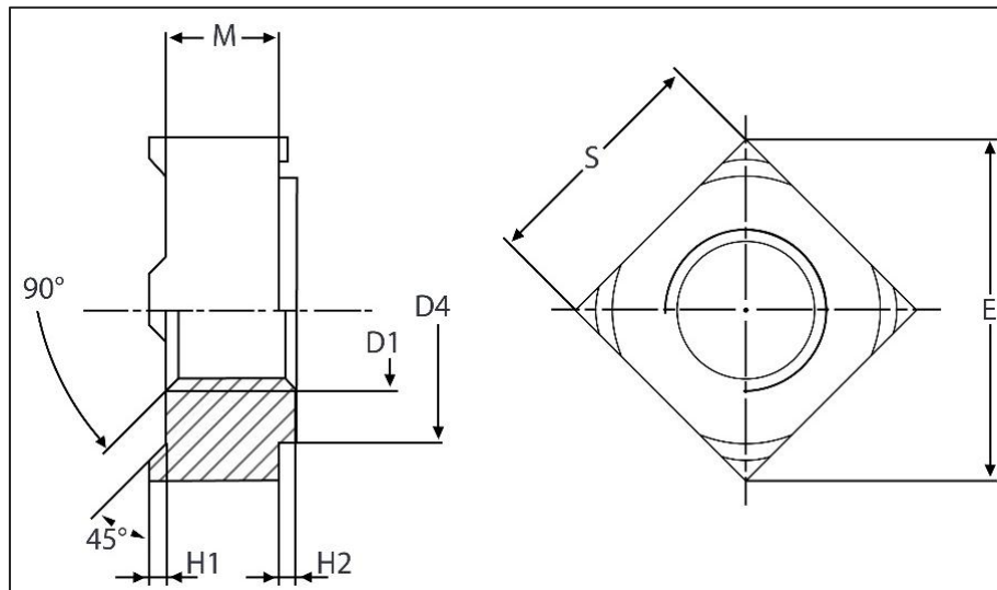
Weight Chart – DIN 928 Square Weld Nut
