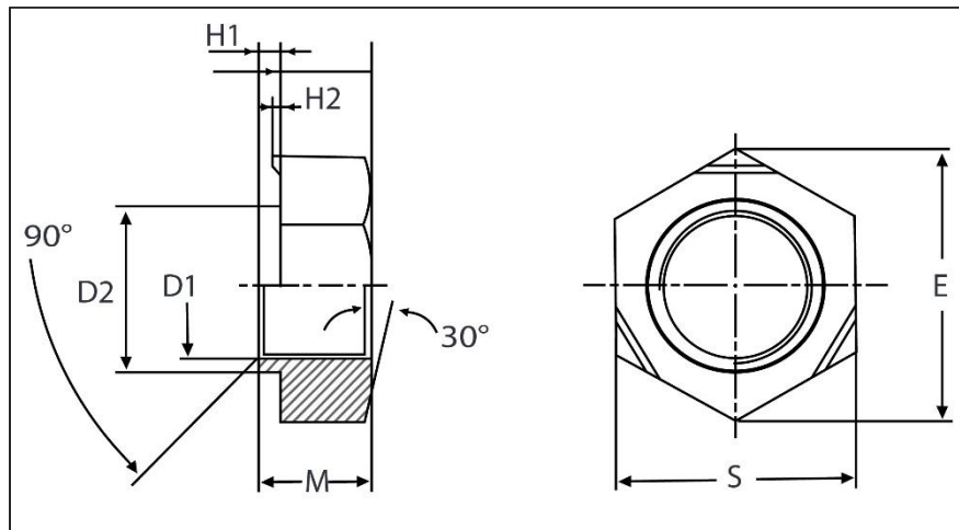
Weight Chart – DIN 929 Hexagon Weld Nut
