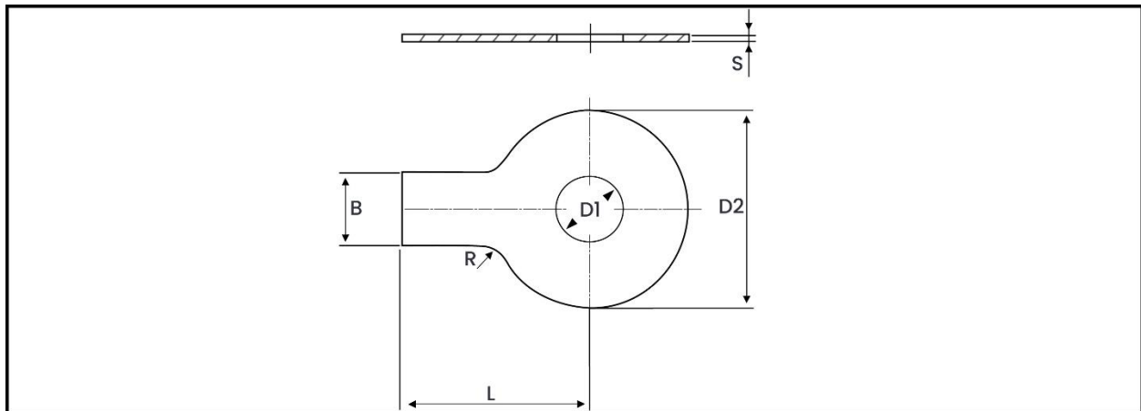
Weight Chart – DIN 93 Tab Washer with Long Tab
