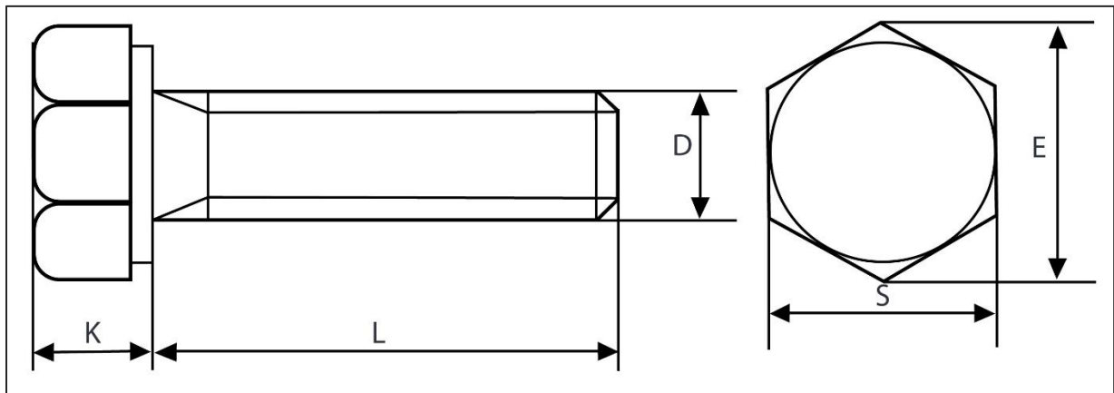
Weight Chart – DIN 933 Hexagon Head Bolt (Fully Threaded)
