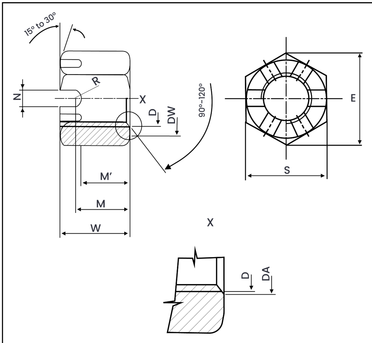
Weight Chart – DIN 935 Slotted Hex Castle Nut
